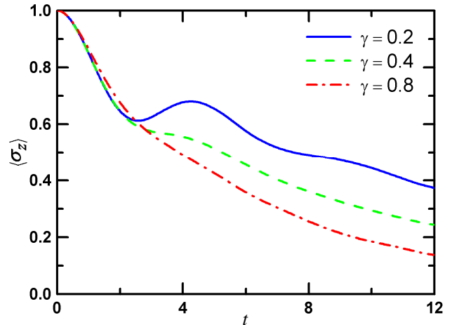
FIG. 1. (color online) Spin state \langle\sigma_z\rangle for various memory parameters: \gamma = 0.2, 0.4, \text{ and } 0.8 . Here \omega = 1 , \Gamma\gamma = 0.2 and \mathcal{N} = 100 .
