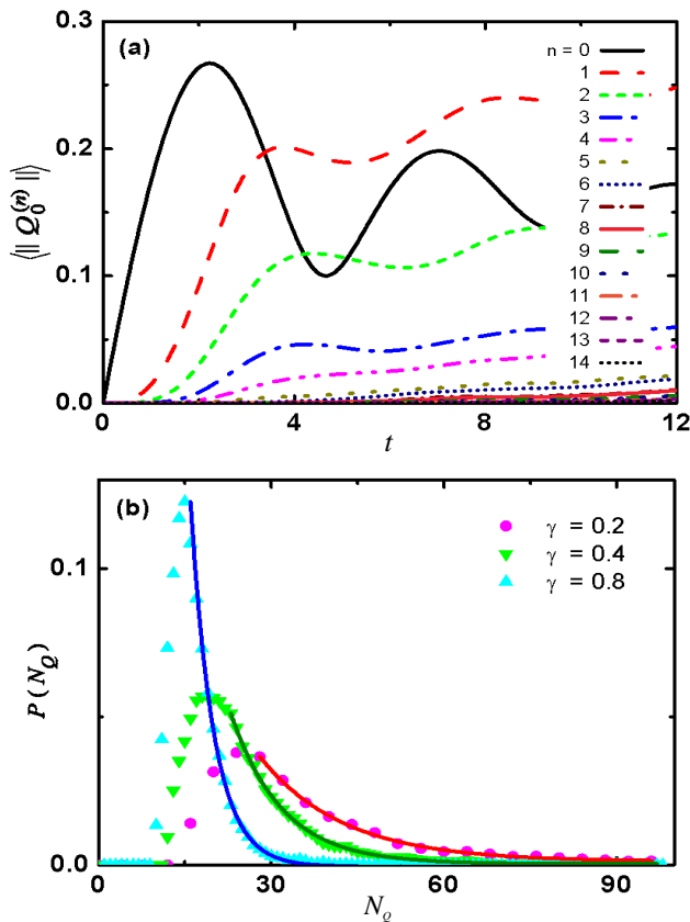
FIG. 3. (color online) (a) Average \langle \|\mathcal{Q}_0^{(n)}\| \rangle of the trace norm of perturbative terms \mathcal{Q}_0^{(n)} from the simulation in Fig. 1 for \gamma = 0.2 . (b) The probability density P(N_Q) of N_Q at t = 12 from the simulations in Fig. 1 for \gamma = 0.2, 0.4 , and 0.8 . Solid lines show fits to exponential distributions for the tails of the distributions.
