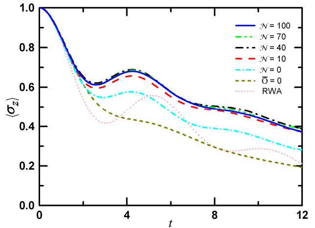
FIG. 2. (color online) Spin state \langle\sigma_z\rangle for \mathcal{N} = 100, 70, 40, 10, \text{ and } 0 , \bar{O} = 0 , and RWA. Here \gamma = 0.2 and \Gamma\gamma = 0.2 .
